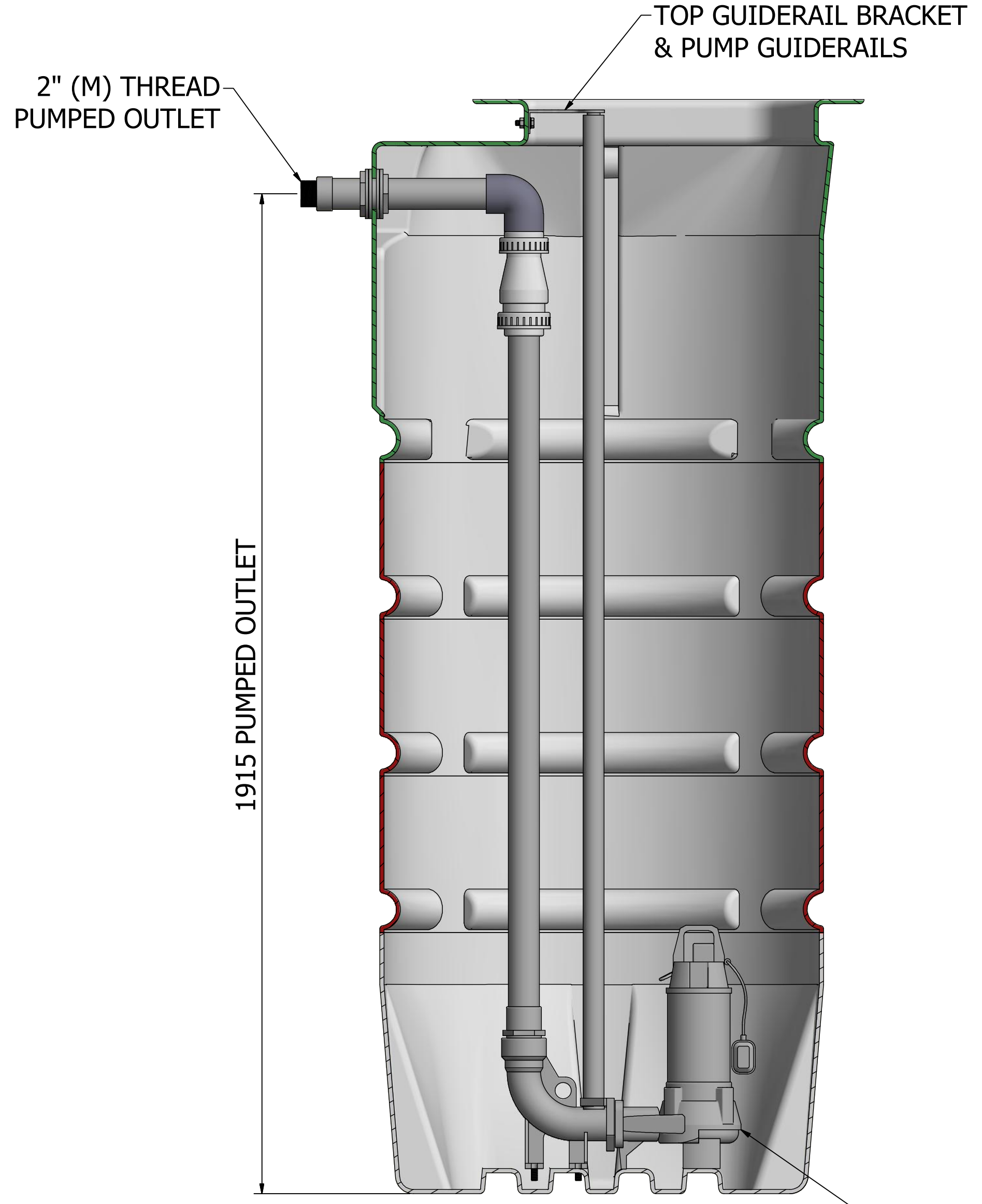
SECTION A-A SCALE 1:7.5
