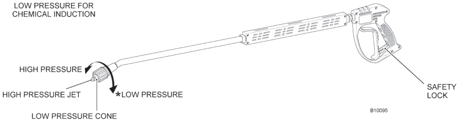
FIXED SINGLE LANCE WITH ADJUSTABLE NOZZLE
