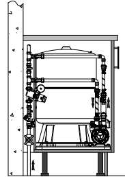
Typical installation Mains Boost Extra 60 (in cupboard)
