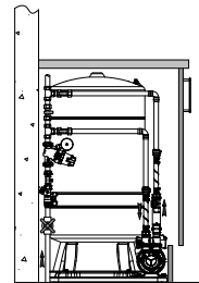
Typical installation Mains Boost Extra 80 (in cupboard on the floor)
