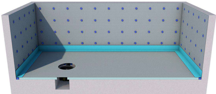
3. Floor insulation applied and covered with membrane and tape.
